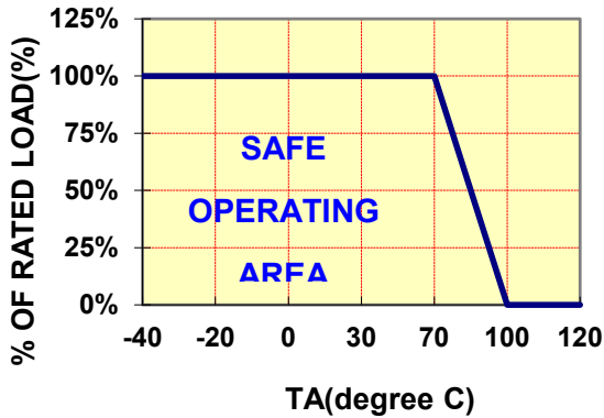
DERATING CURVES
